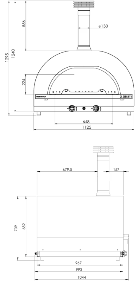
Camera cottura 100x80 cm Peso / Weight 250 kg
